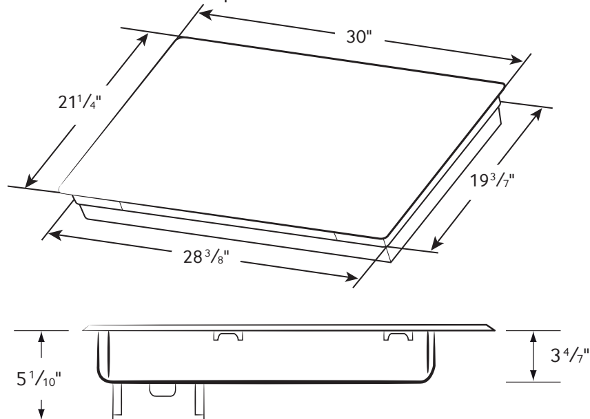
Cooktop Dimensions
